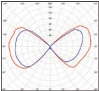
Models 5, 6, 7, 9, 11 E27 (2450 lm) Real light output - 1463 lm
