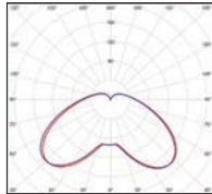
Models 1 to 11 except 3 LED 13W - IP65 Real light output /opal - 384 lm Real light output /clear - 413 lm IRC > 80
