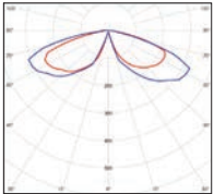
Models 1, 2, 4, 8 E27 (2450 lm) Real light output - 653 lm
