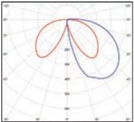
Model 3 LED 13W - IP65 Real light output - 477 lm IRC > 80
