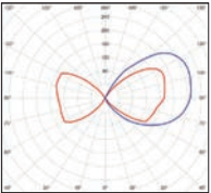
Model 3 E27 (1520 lm) Real light output - 771 lm
