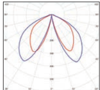
Models 1 to 9 except 2 LED 13W - IP65 Real light output - 361 lm IRC > 80
