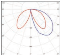
Model 2 LED 13W - IP65 Real light output - 473 lm IRC > 80
